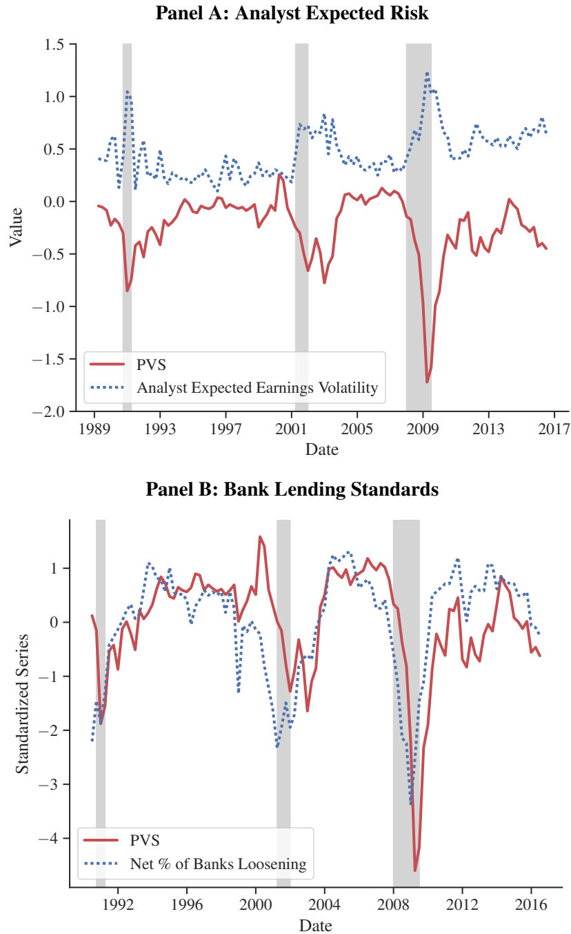
Figure 3: PVS_t and Expected Risk
