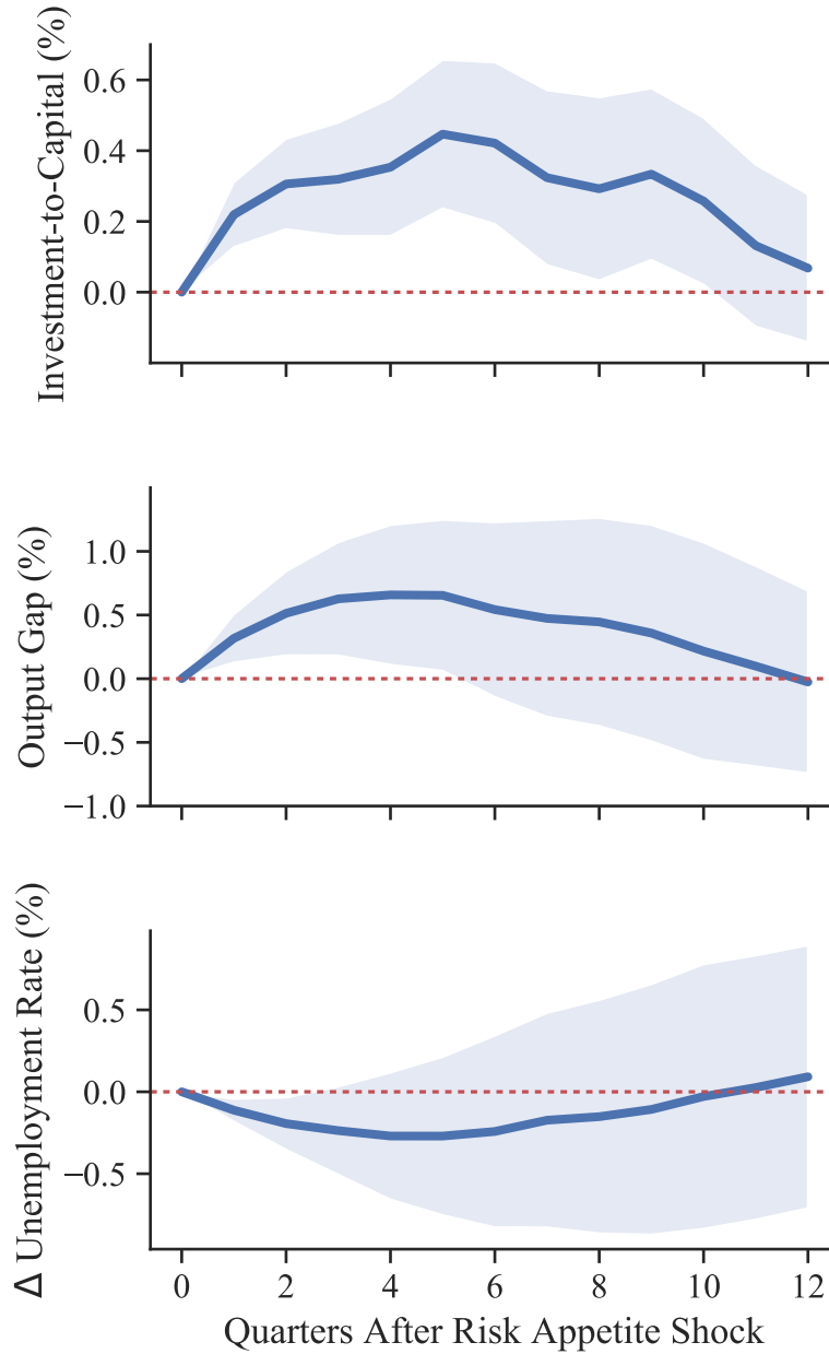
Figure 2: Impulse Responses of the Macroeconomy to PVS Shocks (Local Projections)
